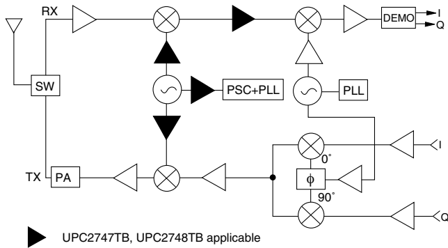
DIGITAL CELLULAR SYSTEM BLOCK DIAGRAM Example of 900 MHz Band Digital Cellular Phone
